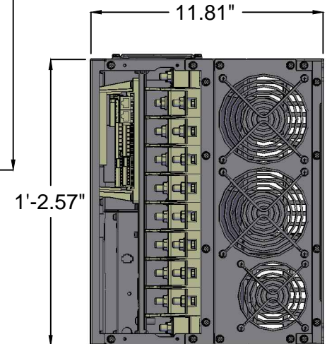
VFD Bottom View
