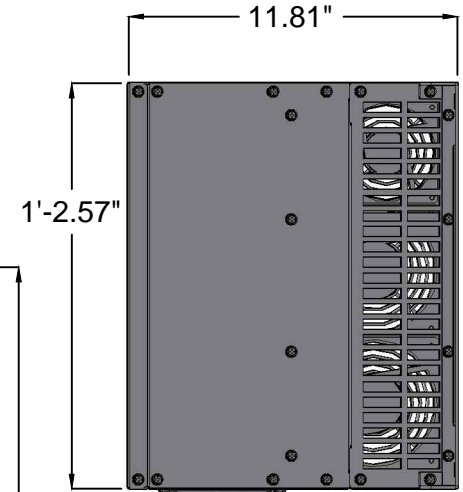
VFD Top View
