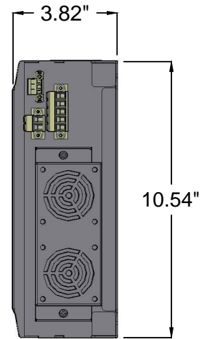
AMBD 10A SPS Bottom View
